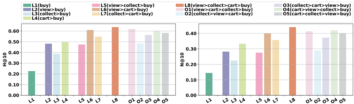
Figure 4: Performance difference of AutoDCS w.r.t. different number and order of behaviors on Jdata. Best viewed in color.
